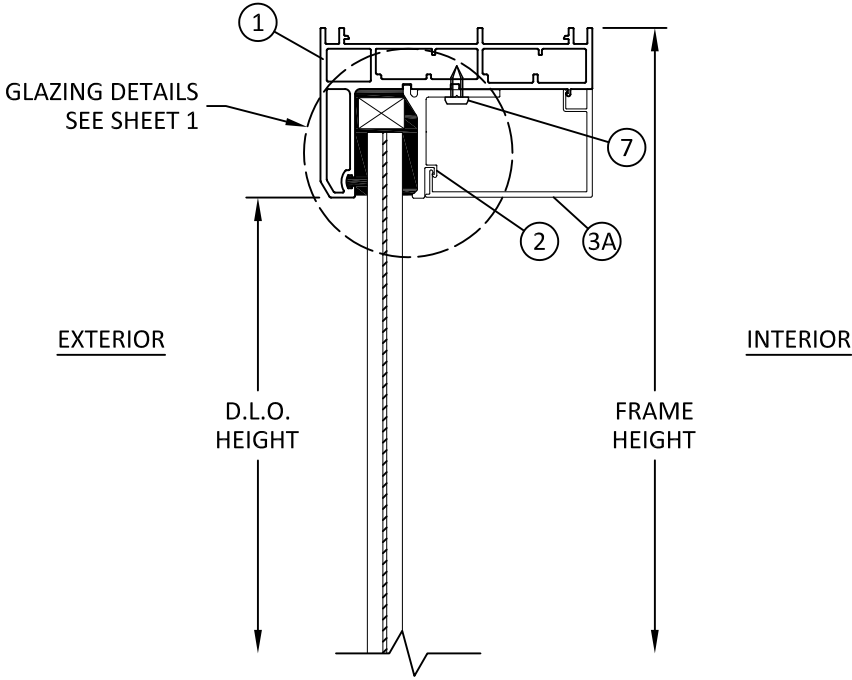
A 4 VERTICAL SECTION HEAD MONOLITHIC GLASS
