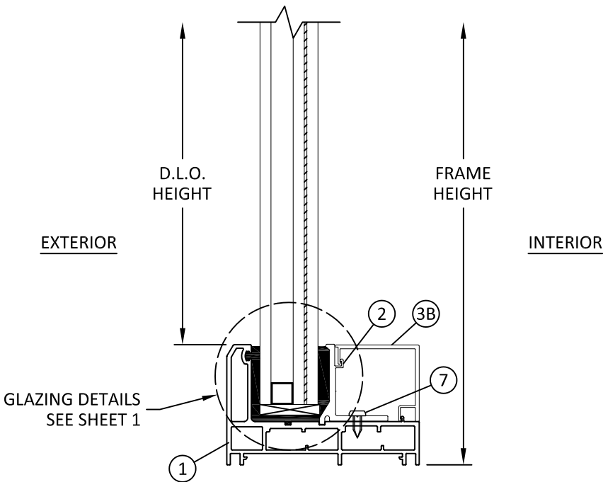
B 4 VERTICAL SECTION SILL INSULATING GLASS
