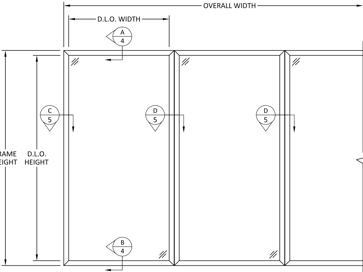
TYPICAL ELEVATION MULLED UNIT
