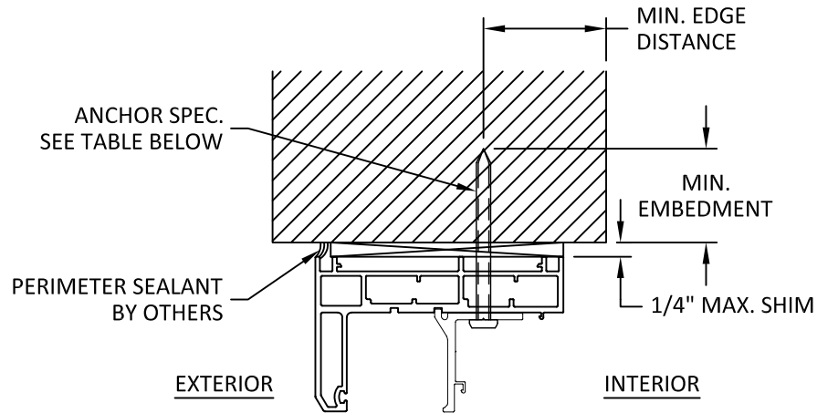
G 6 INSTALLATION DETAIL INSULATING GLASS HEAD SHOWN, JAMB & SILL SIMILAR
