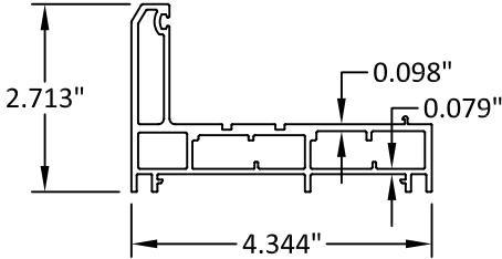
① FRAME HEAD/JAMB/SILL
