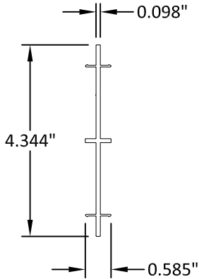
④ MULLION
