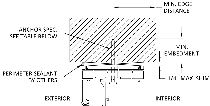
F 6 INSTALLATION DETAIL MONOLITHIC GLASS HEAD SHOWN, JAMB & SILL SIMILAR
