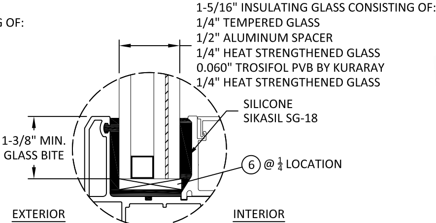
GLAZING DETAIL B SMALL MISSILE IMPACT
