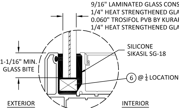
GLAZING DETAIL A SMALL MISSILE IMPACT
